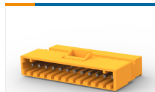
TE Part # 4-641435-2 12P MTA156 CONN ASSY ORNG FRAME
